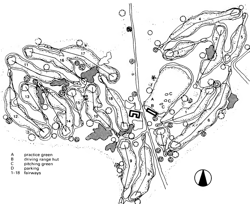
5 Eighteen hole course of normal competition size
